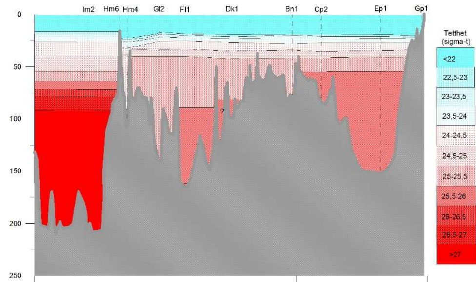
Tetthet (sigma-t) august 2017
